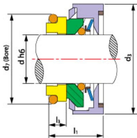
TS XA-20(old)
