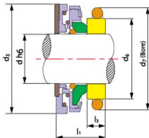
TS XA-25,35,20(new)
